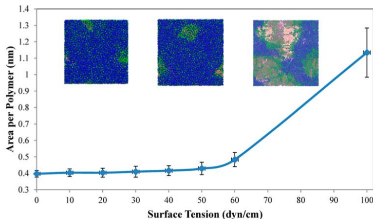
Figure 1. Area per polymer for the L44 (PEO 10 PPO 23 PEO 10 ) block copolymer monolayer at different surface tension values with snapshots of the monolayer taken perpendicular to the membrane normal at the three high surface tension values (50, 60, and 100 dyn/cm) illustrating the membrane rupture and high area per polymer as the surface tension increases. 3
